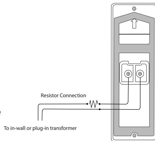
Figure 4: Resistor Connection to in-wall or plug-in transformer
