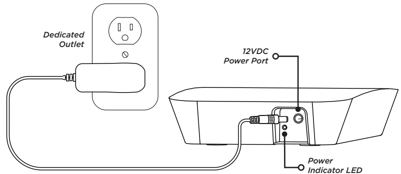
Figure 1: XTLplus-GW Power Connection
