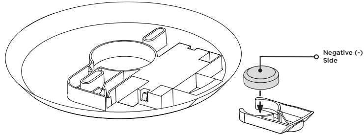
Figure 4: Inserting the Battery
