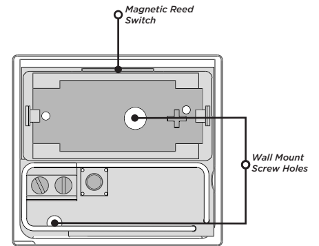
Figure 2: Transmitter Components
