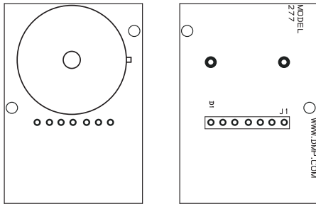
Figure 1: 277CAN Trouble Sounder Front and Rear Views
