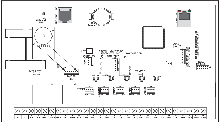
Figure 2: 277CAN Trouble Sounder to Panel Connections
