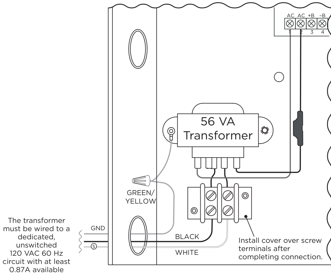
Figure 4: Transformer Wiring
