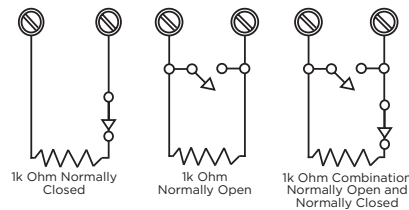
Figure 10: Protection Zone Wiring
