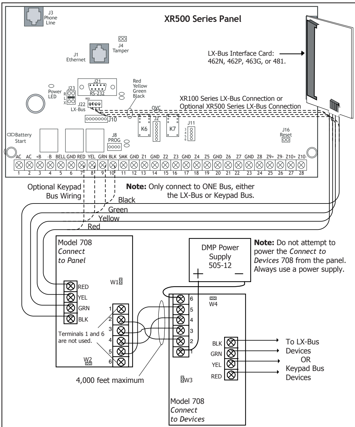
Figure 4: 708 Module Wiring Diagram
