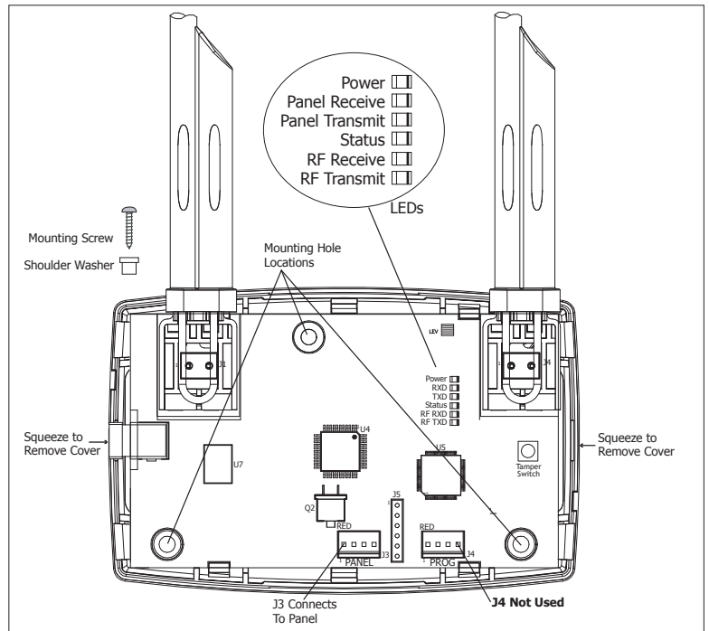
Figure 1: Receiver PCB
