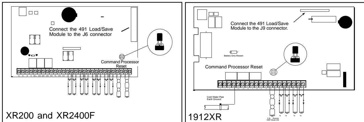
Figure 1: Interface header locations on XR200, XR2400F, and 1912XR panels
